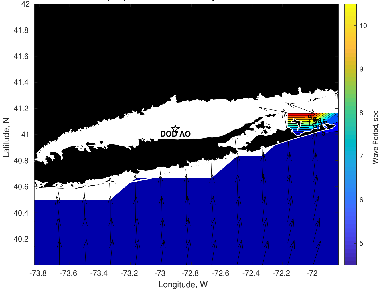
Wave Period (sec) for DOD AO at 03-May-2024 00:00:00
