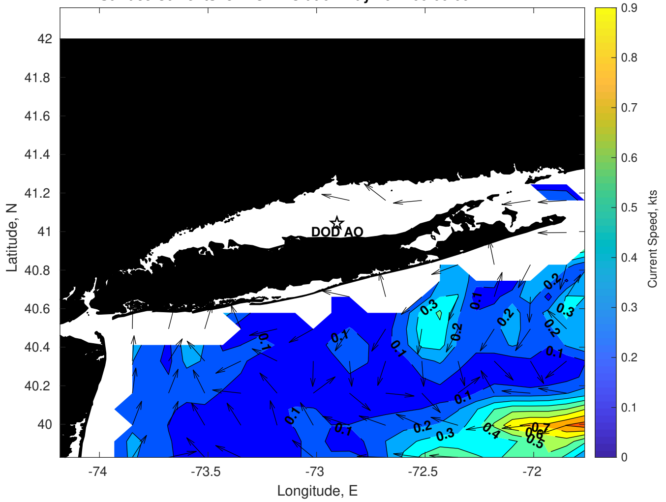
Surface Currents for DOD AO at 02-May-2024 00:00:00
