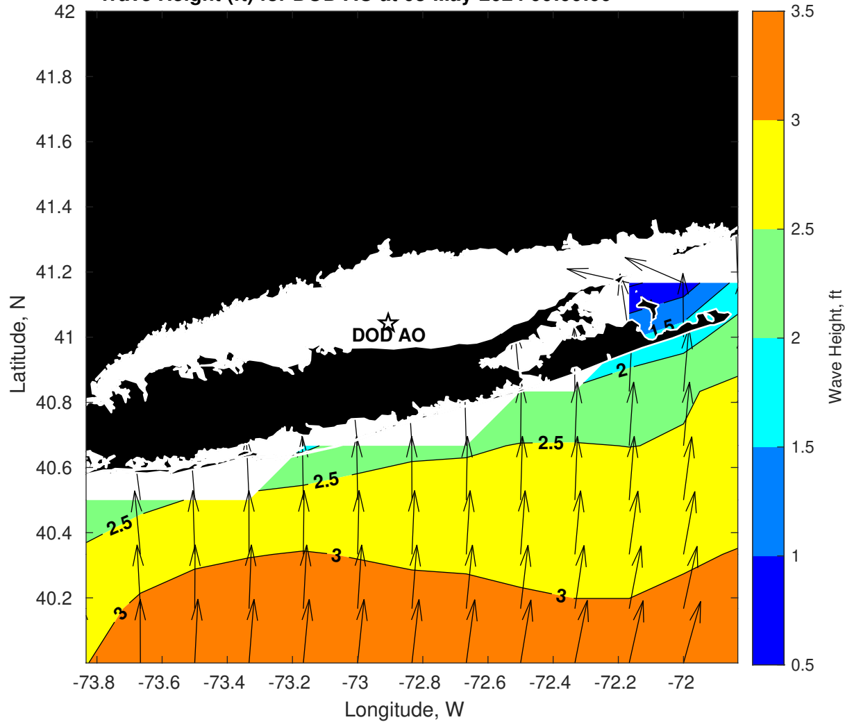
Wave Height (ft) for DOD AO at 03-May-2024 00:00:00
