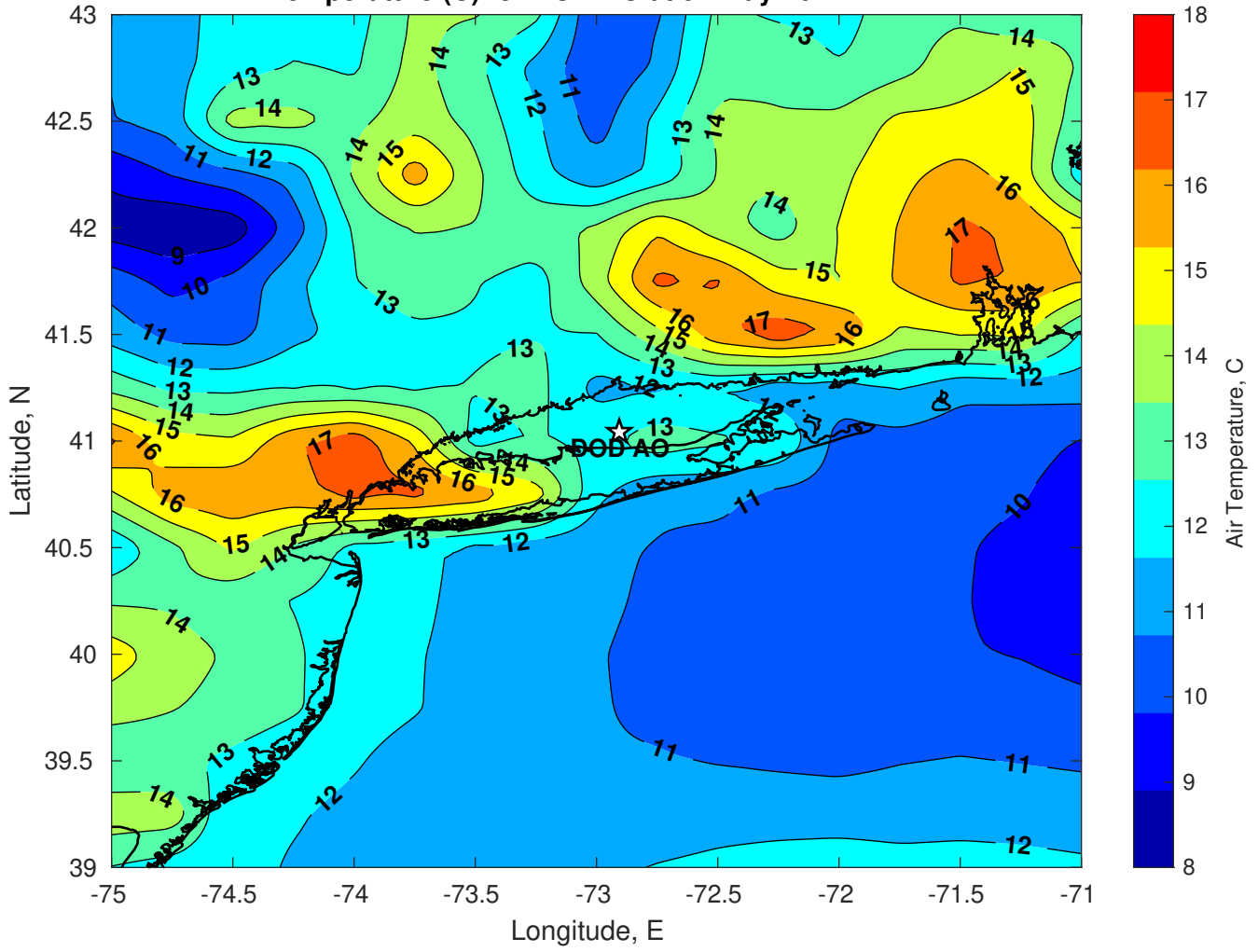
Air Temperature (C) for DOD AO at 02-May-2024
