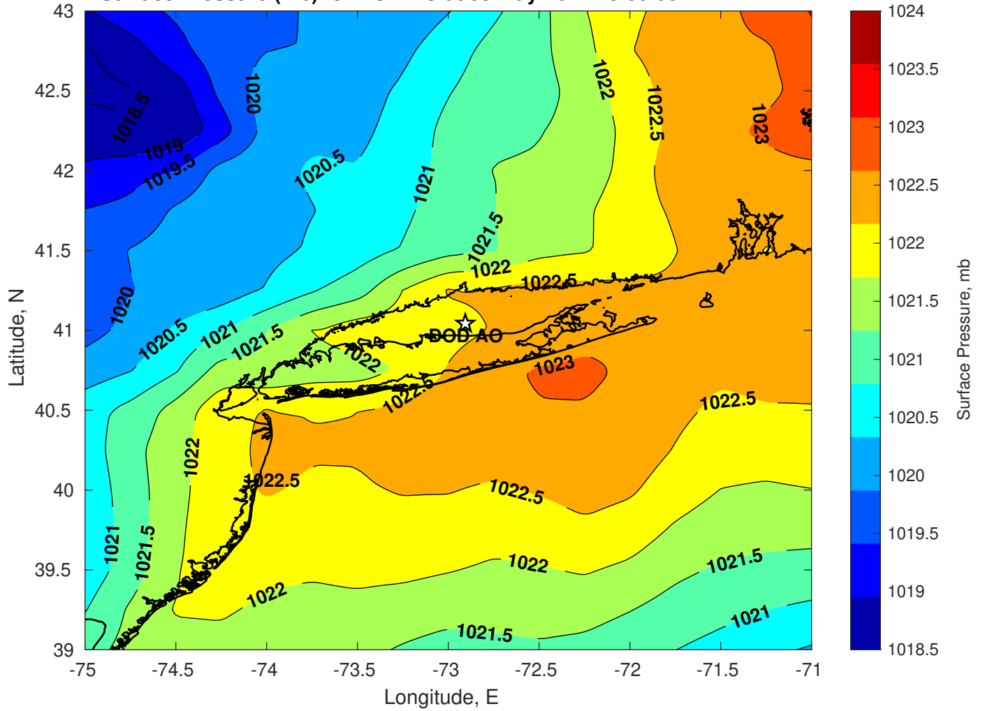
Surface Pressure (mb) for DOD AO at 03-May-2024 18:00:00
