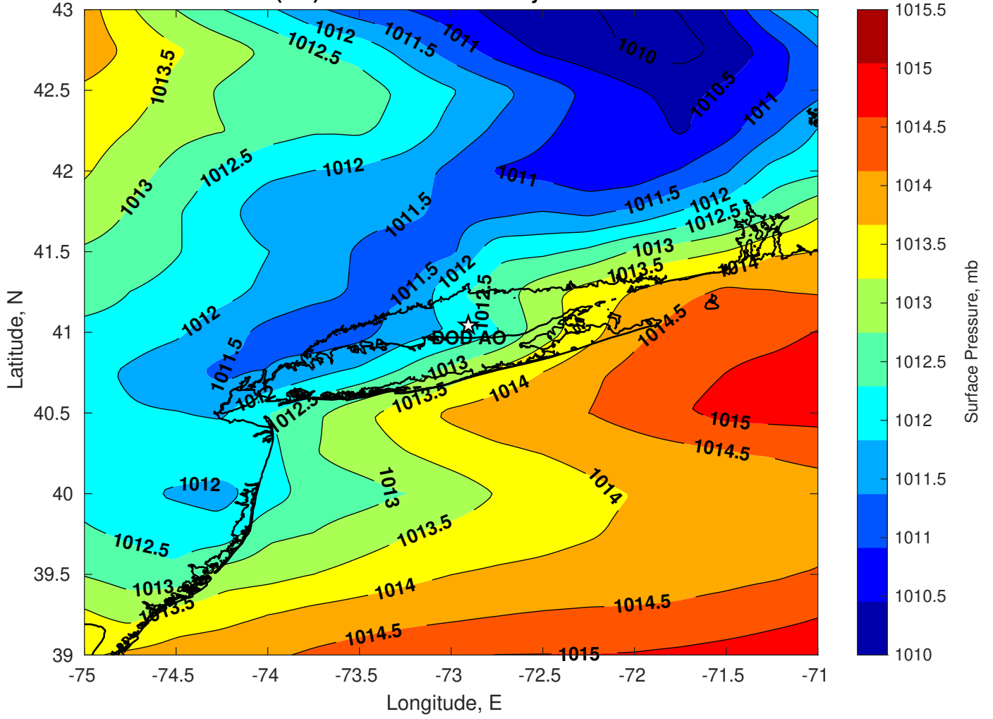
Surface Pressure (mb) for DOD AO at 02-May-2024 18:00:00
