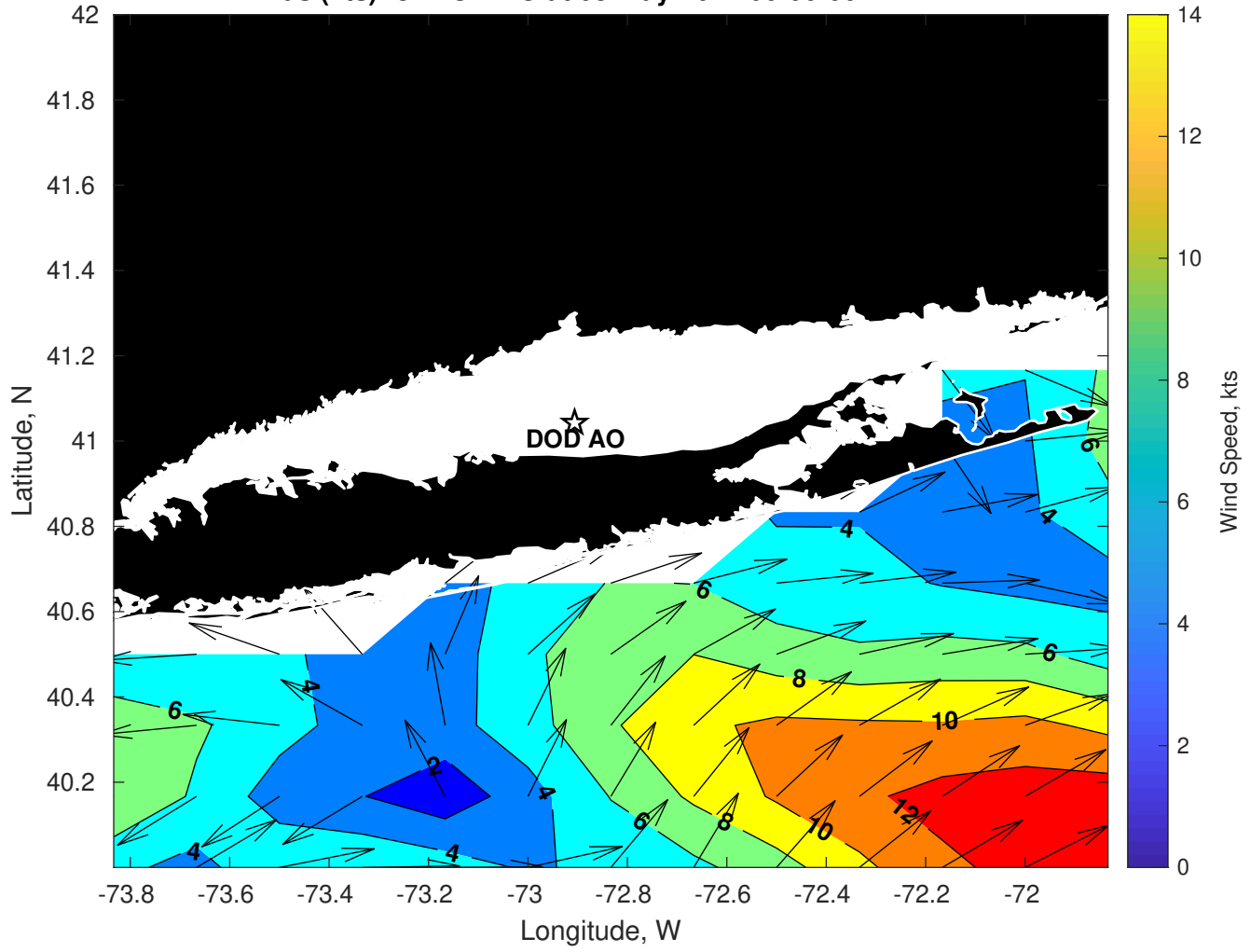
Winds (kts) for DOD AO at 03-May-2024 00:00:00
